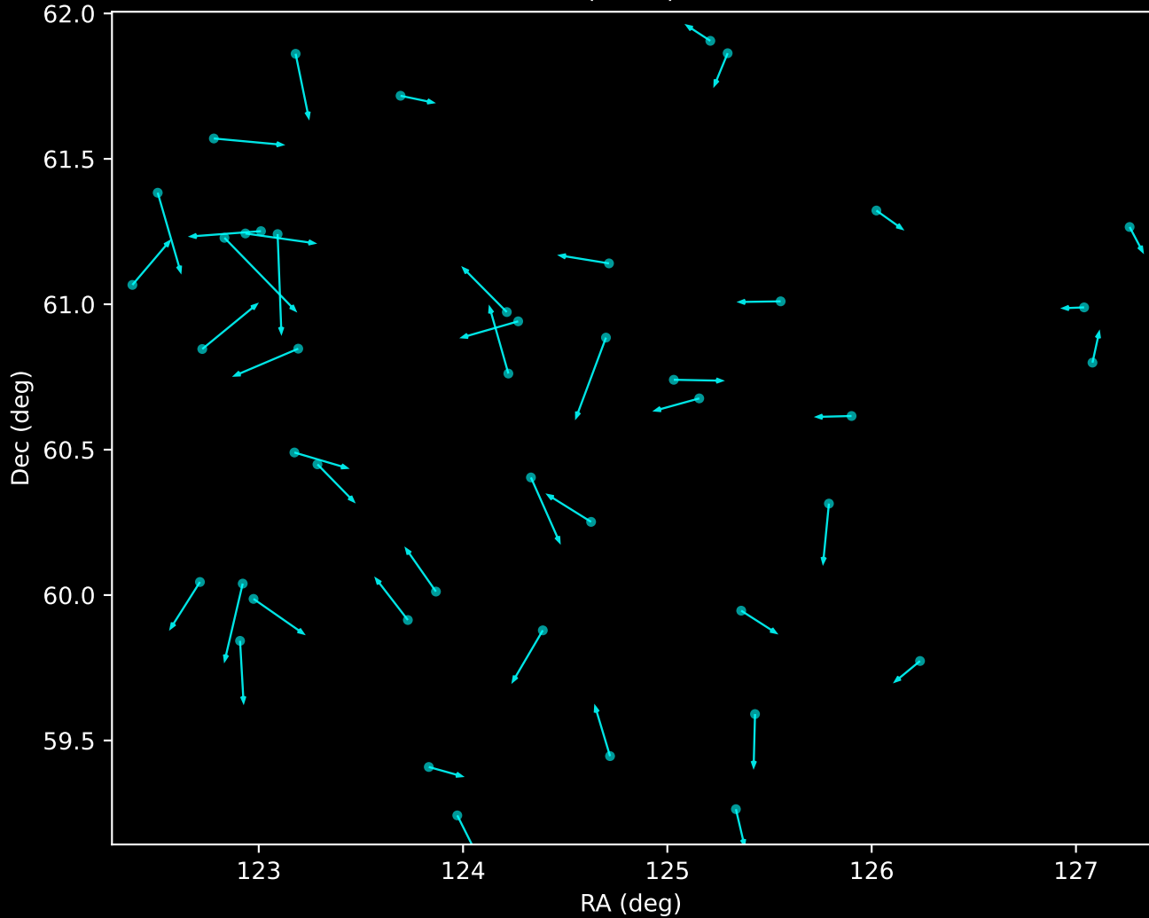
APOGEE DR17 Noise Stream Proper Motion Vectors (n=45)
