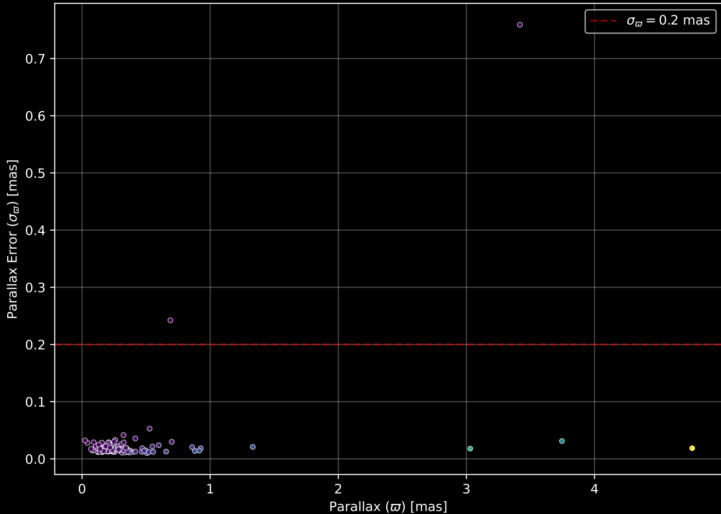
APOGEE DR17 Field: [Cas_S] Parallax Quality (n= 131)
