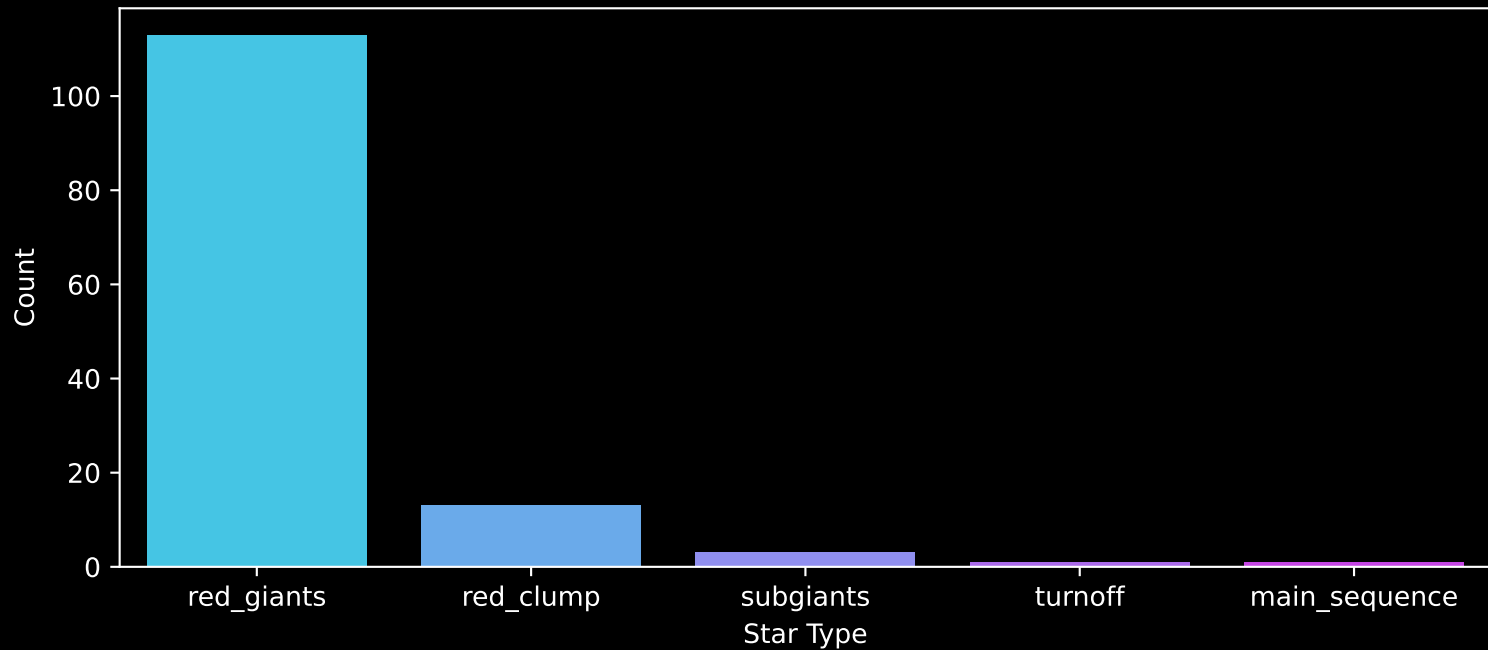
APOGEE DR17 Field: [Cas_S] Count plot of Star Type
