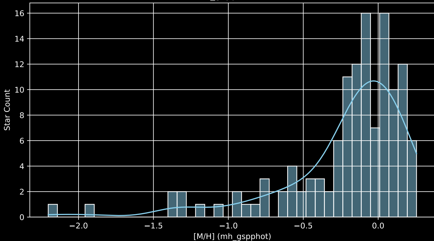
APOGEE DR17 Field: [Cas_S [M/H] (mh_gspphot) (n= 127)
