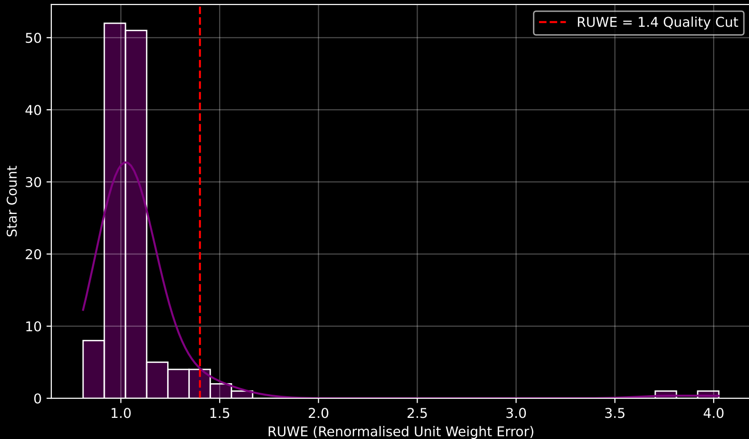
GAPOGEE DR17 Field [Cas_S] RUWE Distribution (n= 129)
