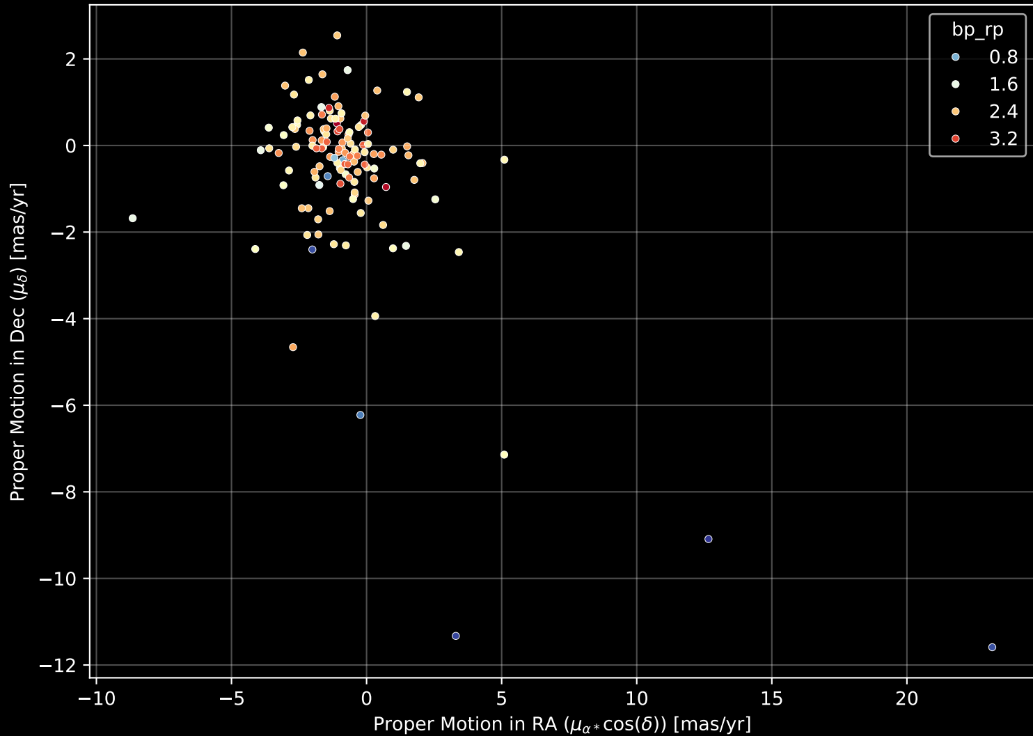
APOGEE DR17 Field: [Cas_S] Proper Motion Diagram (n= 131)
