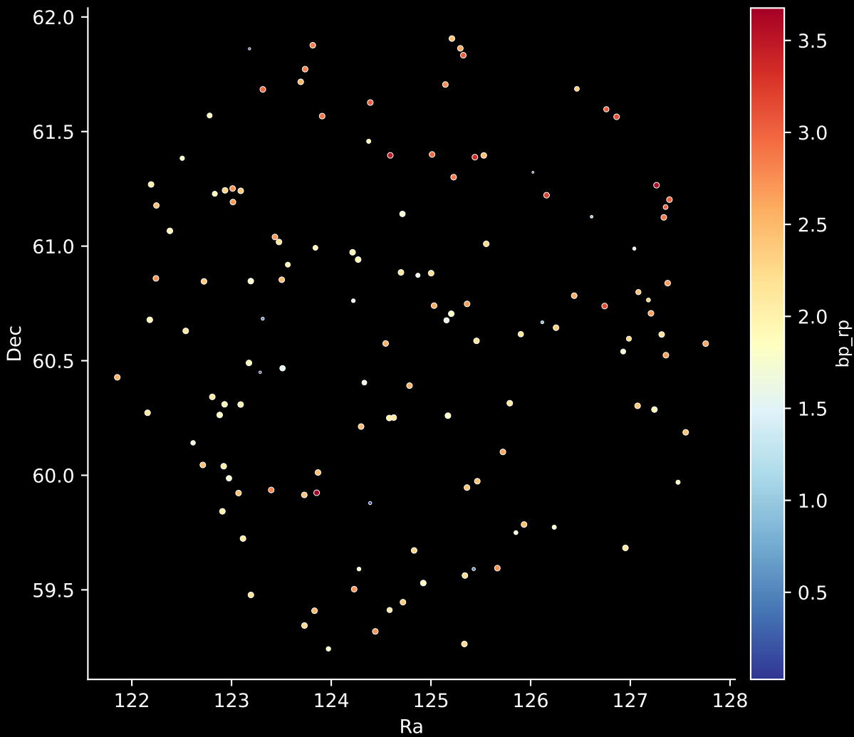
APOGEE DR17 Field: [Cas_S] Stars: 131
