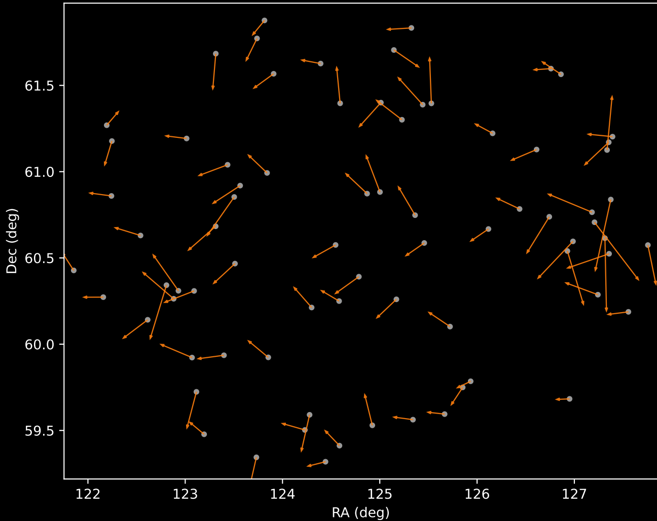
APOGEE DR17 Cluster 2 Proper Motion Vectors (n=76)
